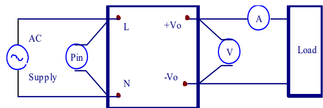
Figure 1. CFM130S Series Test Setup
