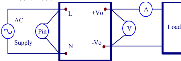
Figure 1. CFM21M Series Test Setup
