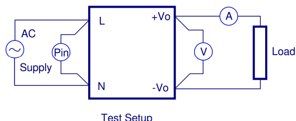
Figure 1. CFM300S Series Test Setup
