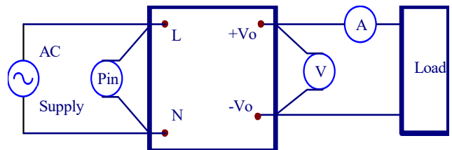
Figure 1. CFM40S Series Test Setup
