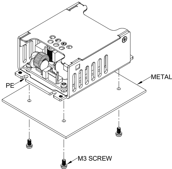
CFM70SXXX-CA installation diagram
