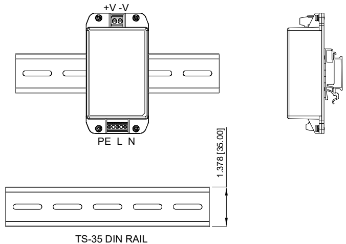
CFM70SXXX-SD installation diagram
