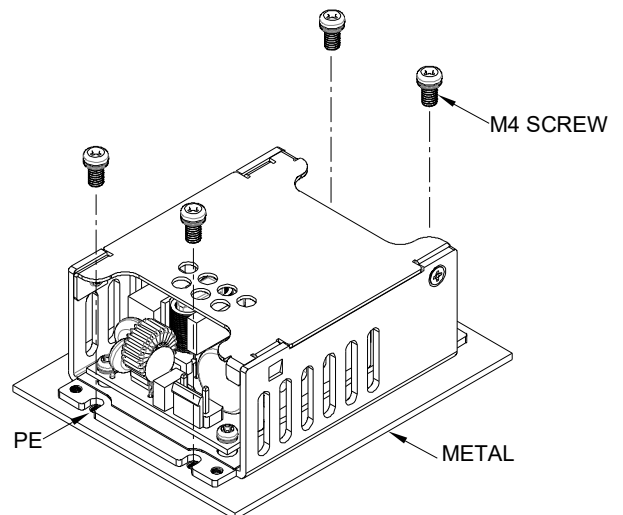
CFM70SXXX-P installation diagram
