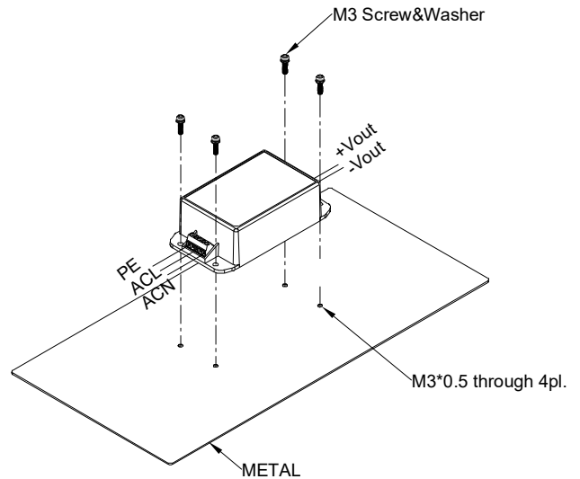
CFM70SXXX-S installation diagram
