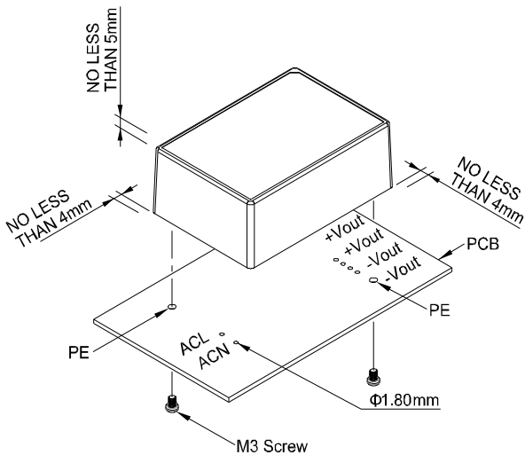
CFM70SXXX-E installation diagram
