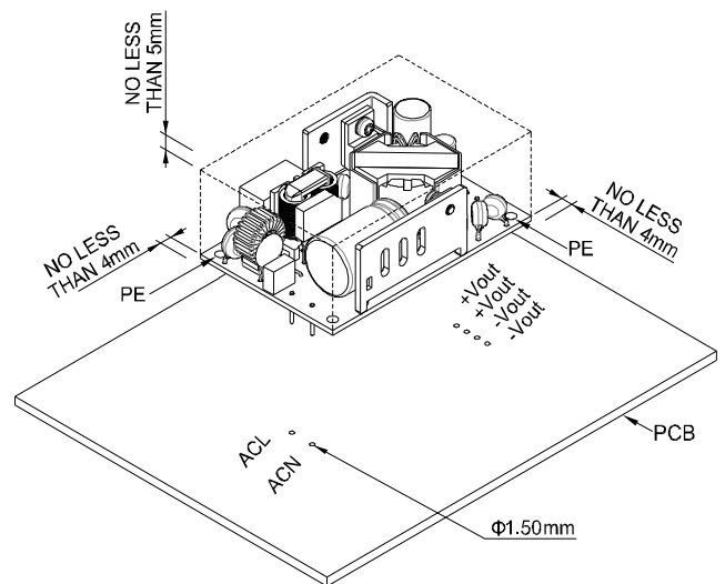
CFM70SXXX-P installation diagram
