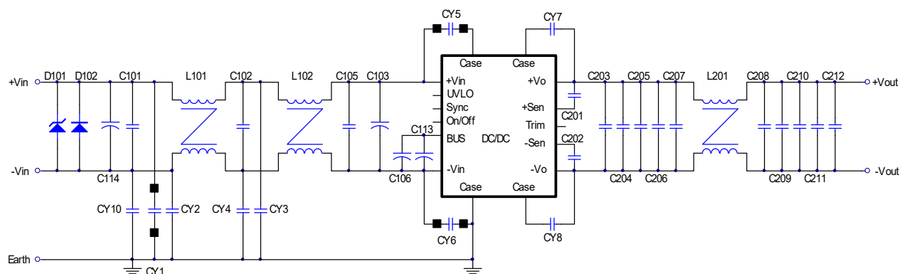
Figure1 Connection Circuit
