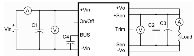
CHB150W12 Series Test Setup
