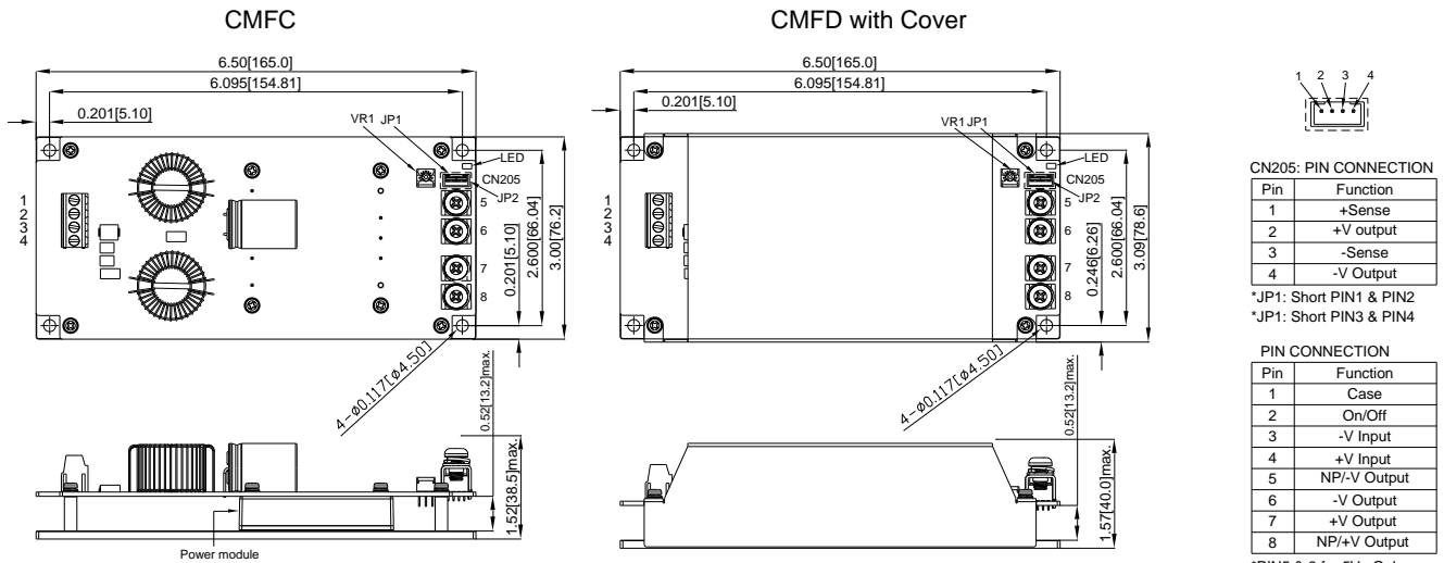
CHB200W-110SXX-CMFC(D) Mechanical Outline Diagram
