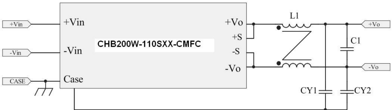
Connection circuit for EMI testing
