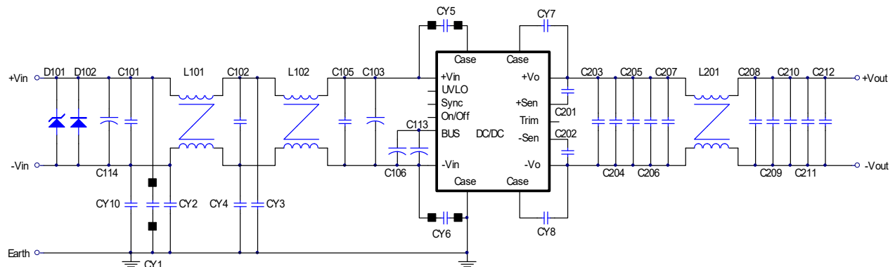
Figure1 Connection Circuit
