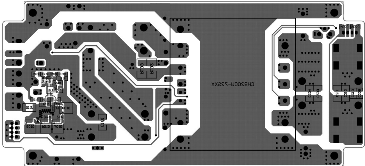
Figure3 PCB Layout Bottom View
