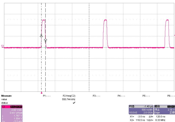
Synchronization pulse width 120ns
