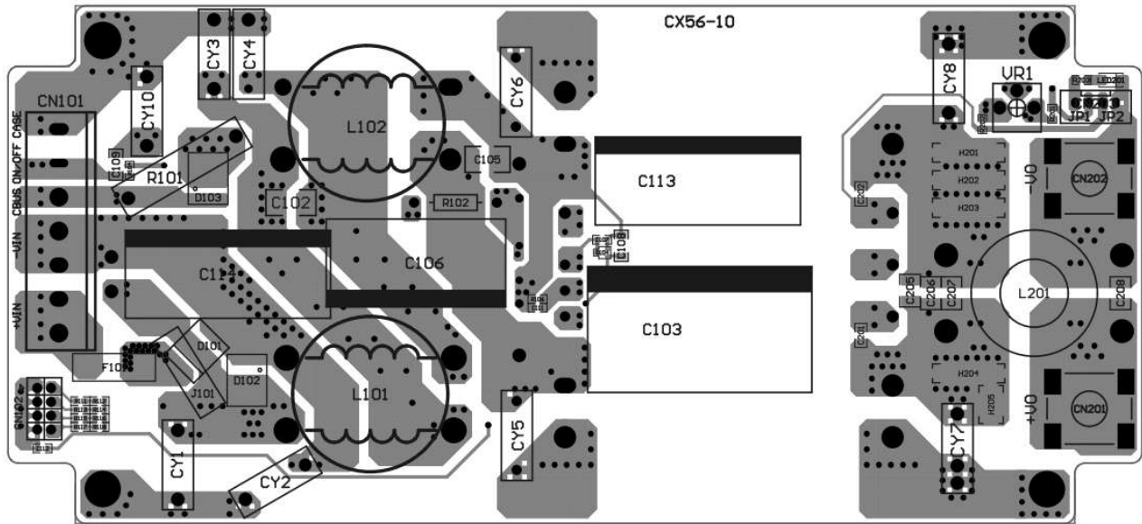
Figure2 PCB Layout Top View
