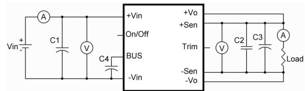
CHB200W12 Series Test Setup
