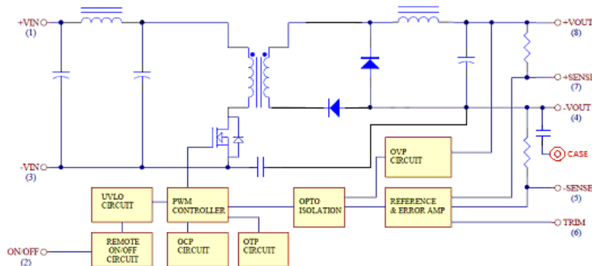
Electrical Block Diagram for other modules
