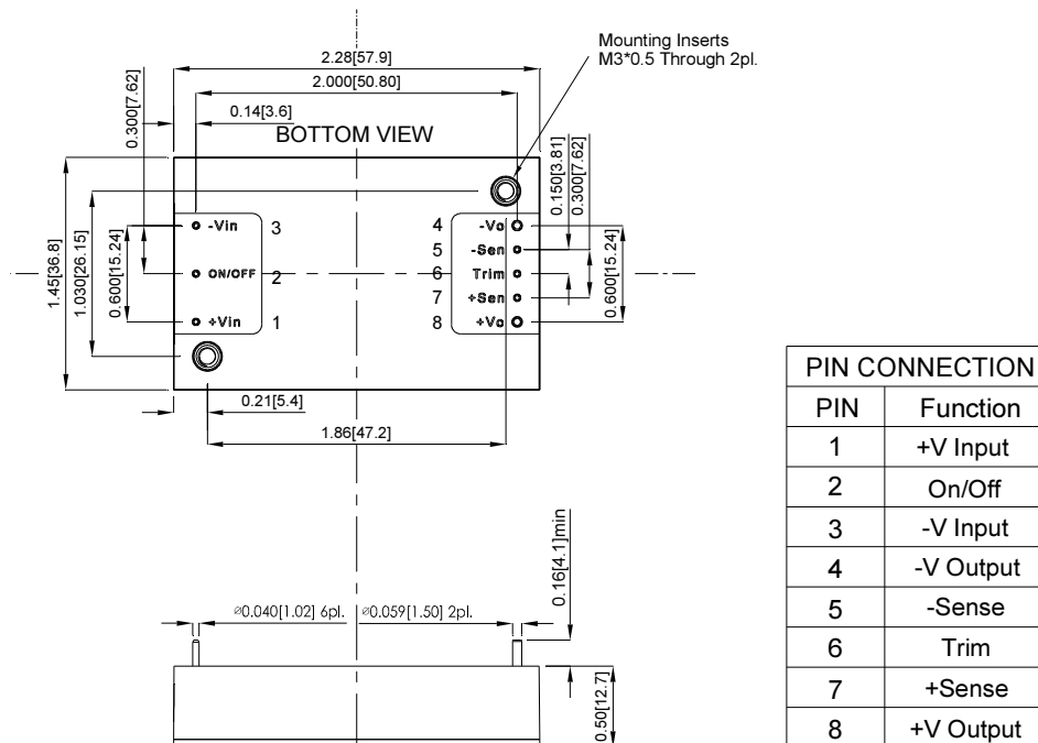
CQB100W-110SXX Mechanical Outline Diagram
