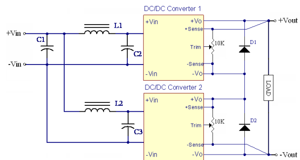
Simple Series Operation Connect Circuit
