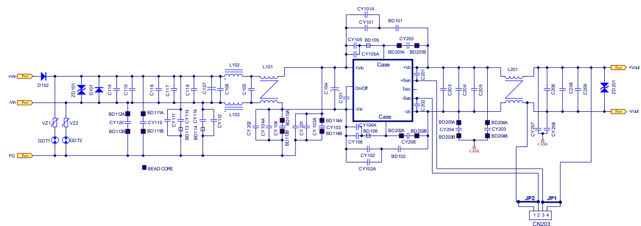
Figure1 Connection Circuit
