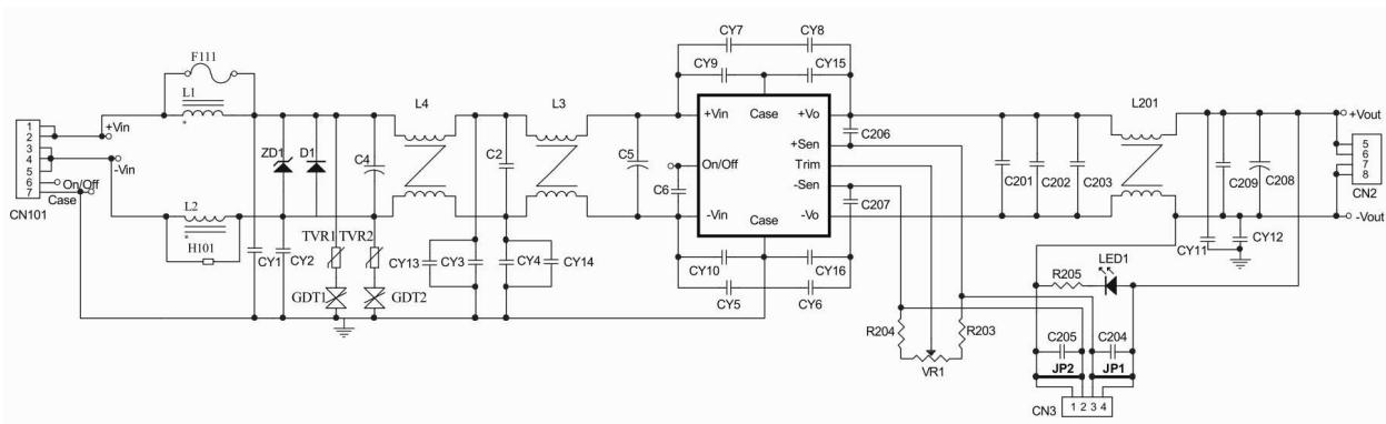
Figure1 Connection Circuit
