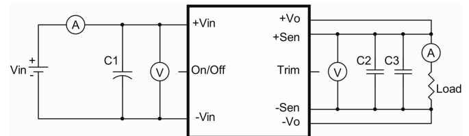
CQB75W14 Series Test Setup
