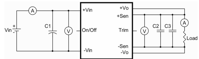
CQB75W14 Series Test Setup
