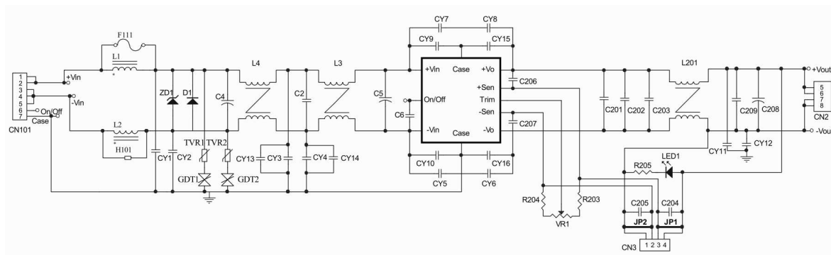
Figure1 Connection Circuit
