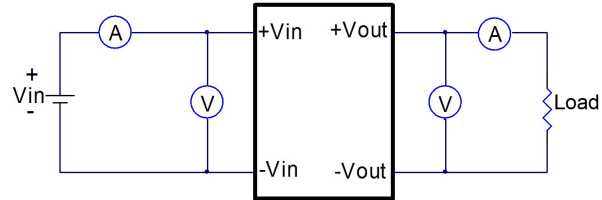
DH45W10 Series Test Setup
