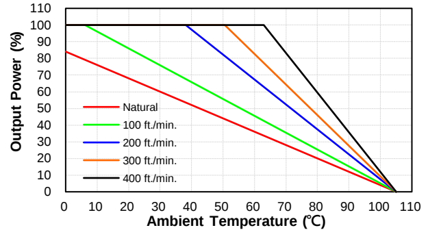
CQB100W14-72S15, 24, 28, 54 Derating Curve without Heatsink (Vin=72V)
