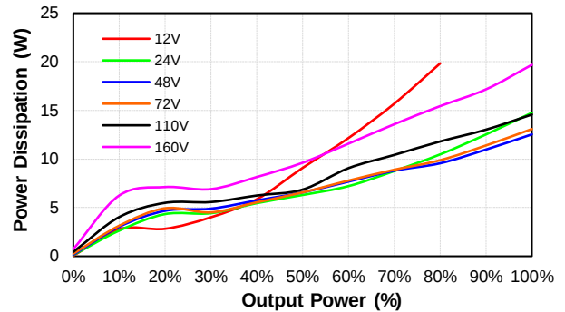
CQB100W14-72S05 Pd Vs Po @25 Deg. C
