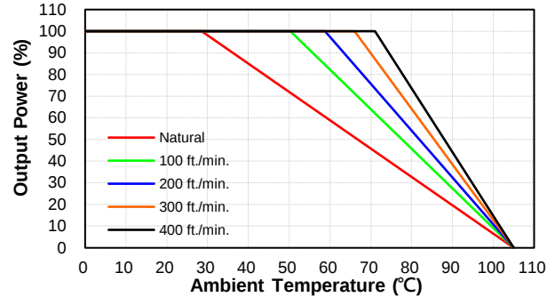
CQB100W14-72S05, 12 Derating Curve with Heatsink QBL127 (Vin=72V)
