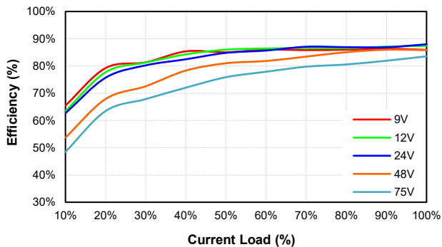
EC3AW8-48D12 Eff Vs Io @25 Deg. C
