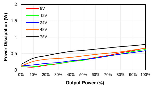
EC3AW8-48S05 Pd Vs Po @25 Deg. C
