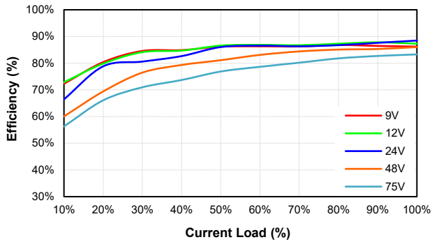
EC3AW8-48S12 Eff Vs Io @25 Deg. C
