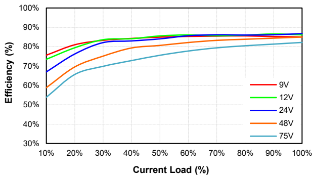
EC3AW8-48S15 Eff Vs Io @25 Deg. C
