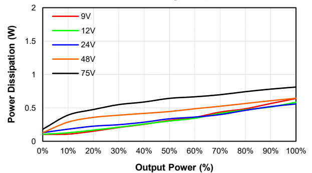
EC3AW8-48D05 Pd Vs Po @25 Deg. C
