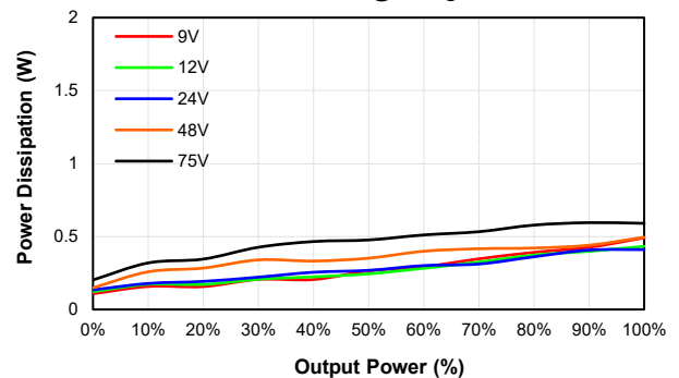
EC3AW8-48D12 Pd Vs Po @25 Deg. C
