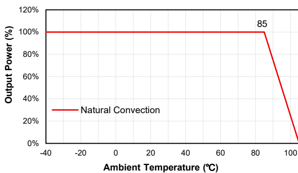
Typical Derating Curve for Natural Convection ( V_{in} =Nominal)
