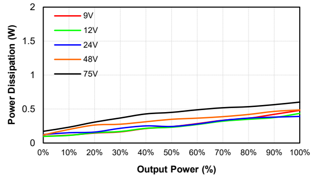
EC3AW8-48S12 Pd Vs Po @25 Deg. C
