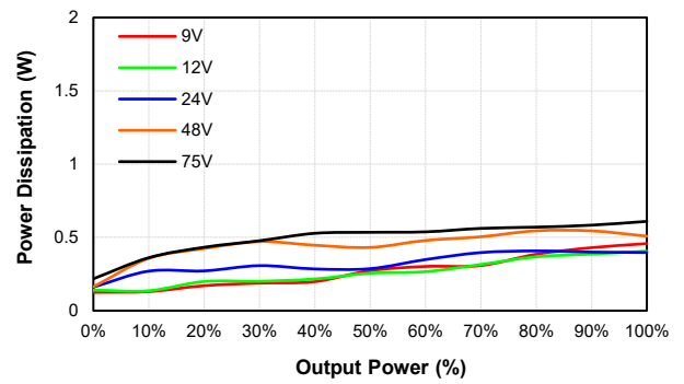
EC3AW8-48D15 Pd Vs Po @25 Deg. C
