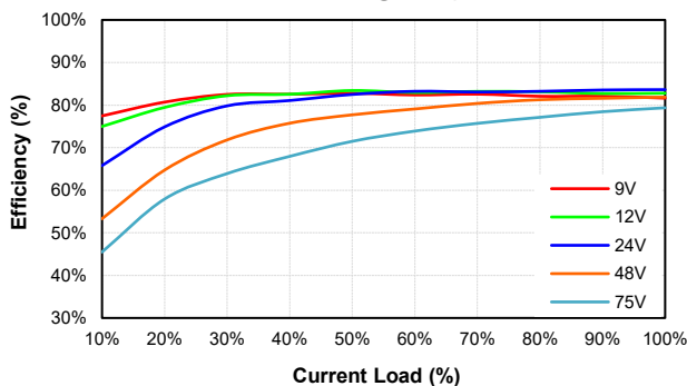
EC3AW8-48S05 Eff Vs Io @25 Deg. C
