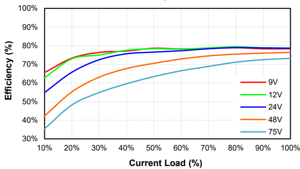
EC3AW8-48S33 Eff Vs Io @25 Deg. C
