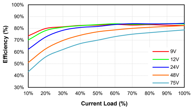
EC3AW8-48D05 Eff Vs Io @25 Deg. C
