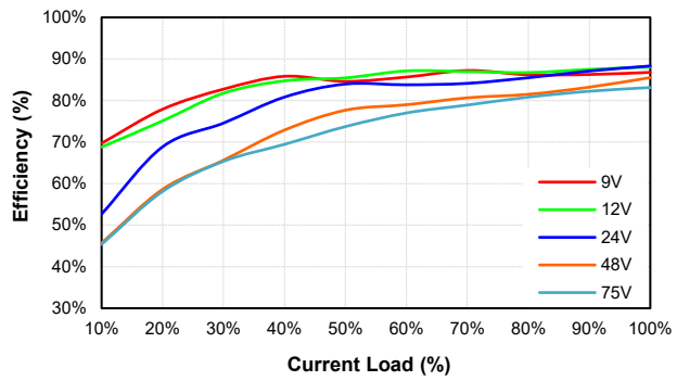
EC3AW8-48D15 Eff Vs Io @25 Deg. C
