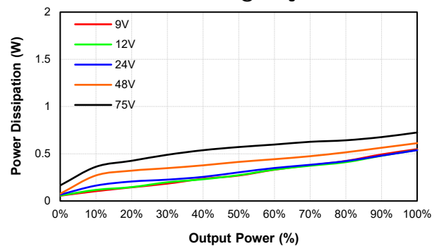
EC3AW8-48S33 Pd Vs Po @25 Deg. C
