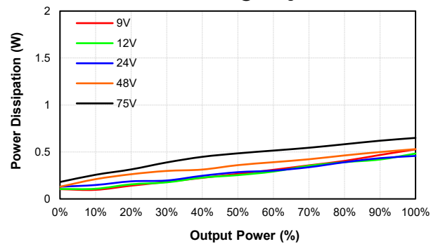
EC3AW8-48S15 Pd Vs Po @25 Deg. C
