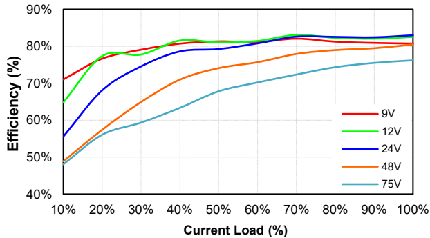
EC4AW8-48D05 Eff Vs Io @25 Deg. C
