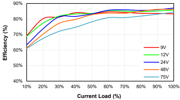
EC4AW8-48S12 Eff Vs Io @25 Deg. C
