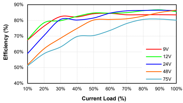
EC4AW8-48D15 Eff Vs Io @25 Deg. C
