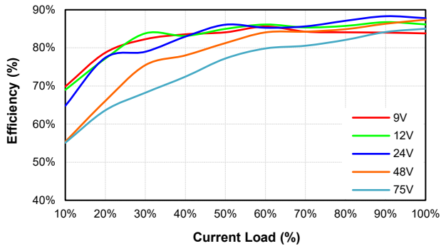
EC4AW8-48S15 Eff Vs Io @25 Deg. C
