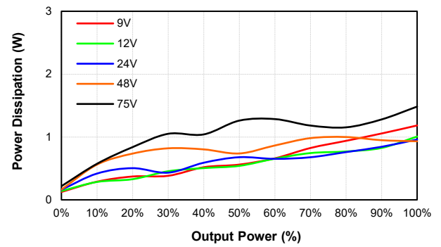
EC4AW8-48D15 Pd Vs Po @25 Deg. C
