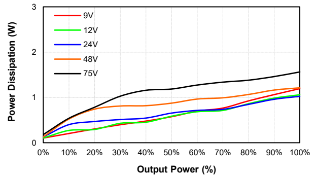
EC4AW8-48D05 Pd Vs Po @25 Deg. C
