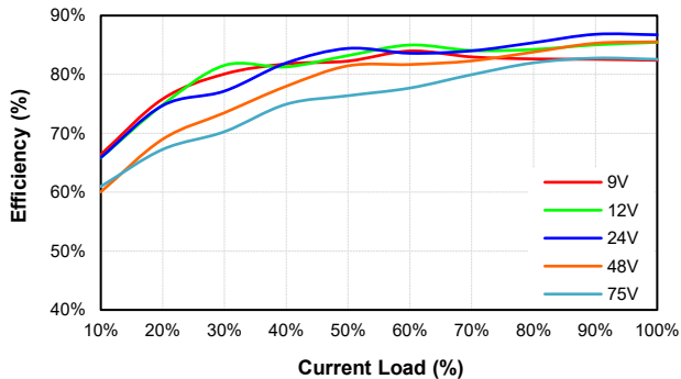
EC4AW8-48D12 Eff Vs Io @25 Deg. C
