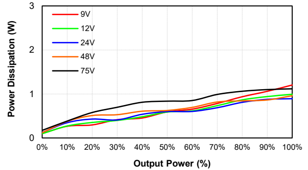
EC4AW8-48S12 Pd Vs Po @25 Deg. C
