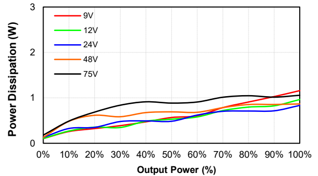
EC4AW8-48S15 Pd Vs Po @25 Deg. C
