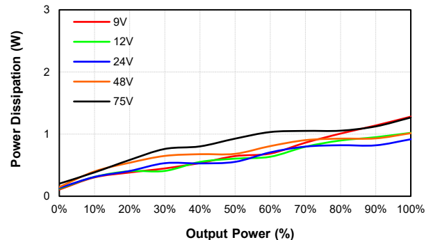
EC4AW8-48D12 Pd Vs Po @25 Deg. C
