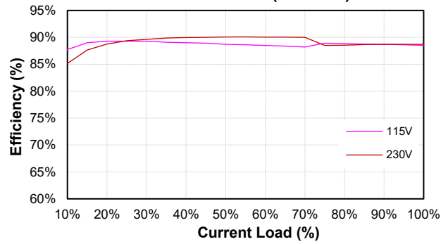
TRH100A135 (Eff Vs Io)
