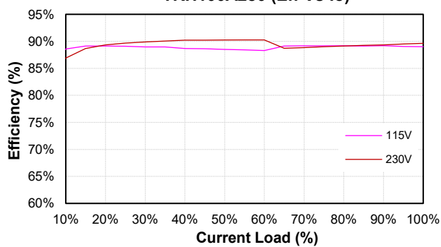
TRH100A280 (Eff Vs Io)
