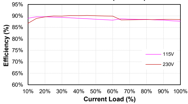
TRH100A120 (Eff Vs Io)
