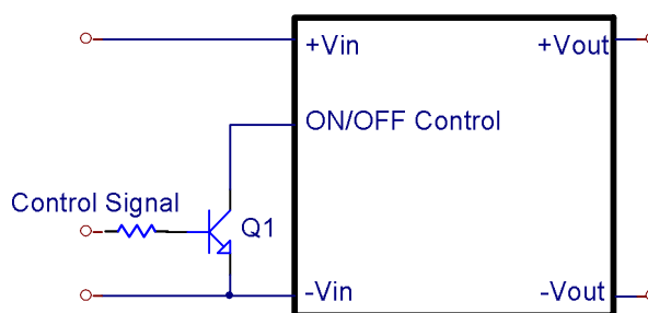
Remote On/Off Input Drive Circuit
