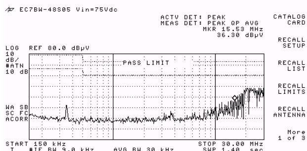
Conducted Emission of EN55032 class A for EC7C-48D12
