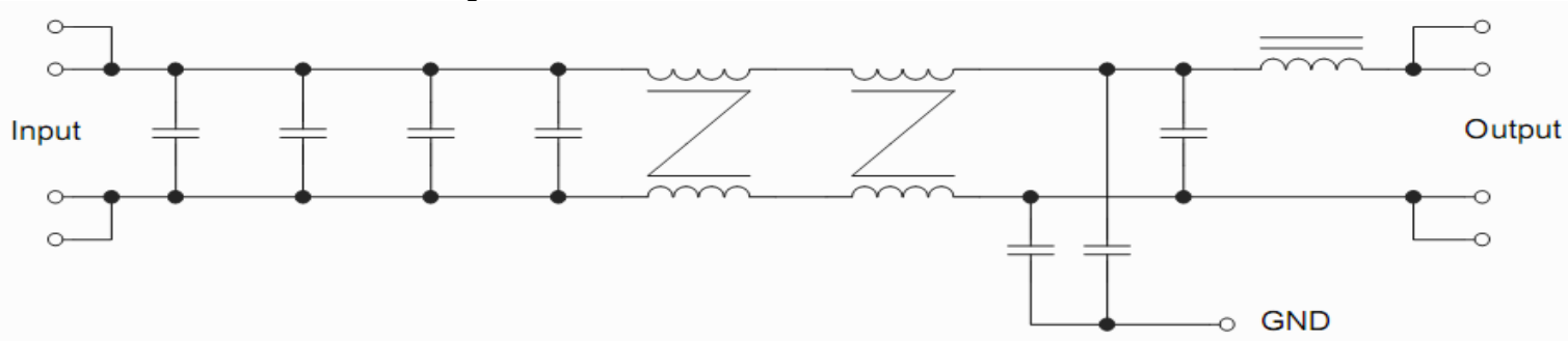
Figure2 Internal Schematic for FM20-100 Module
