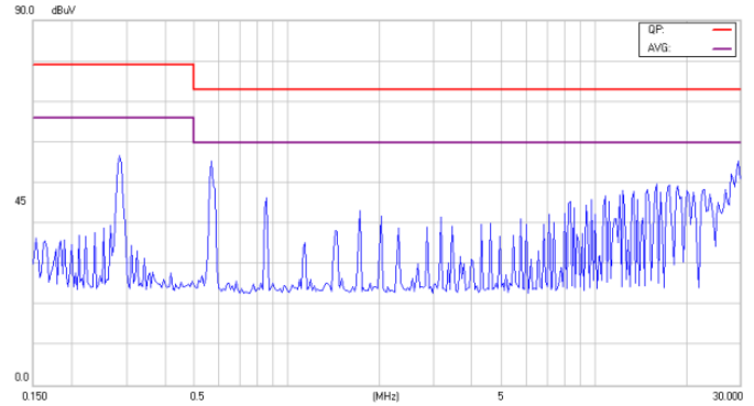
Conducted EN55032 Class A of CQB75W-48S15
