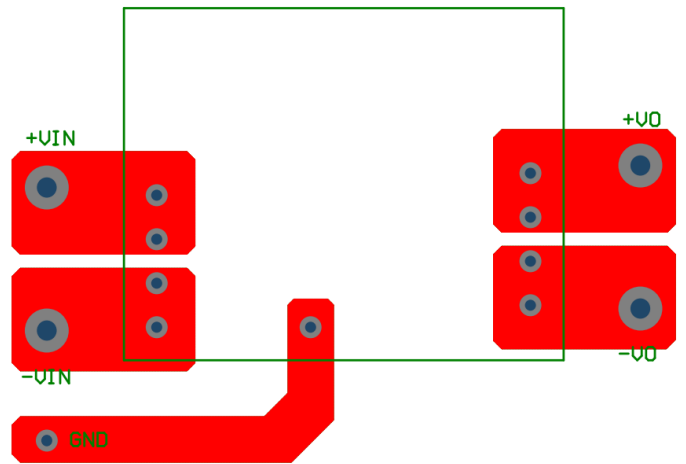
FM20-100 Suggested PCB Layout
