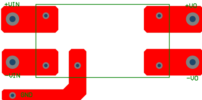
FM10-100 PCB Footprint
