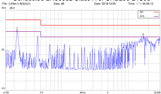
Conducted EN55032 Class A of CHB300W-48S12
