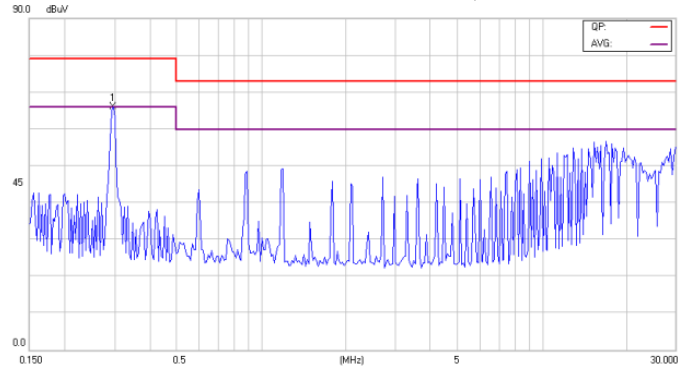
Conducted EN55032 Class A of CHB75-48S15
