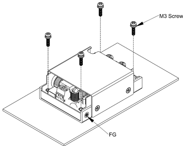
LFM200MXXC Installation Diagram
