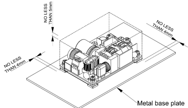
LFM200MXXB Installation Diagram
