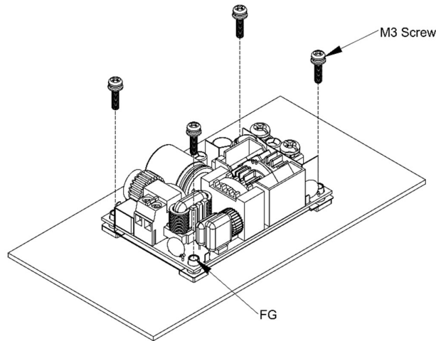
LFM200MXXB Installation Diagram
