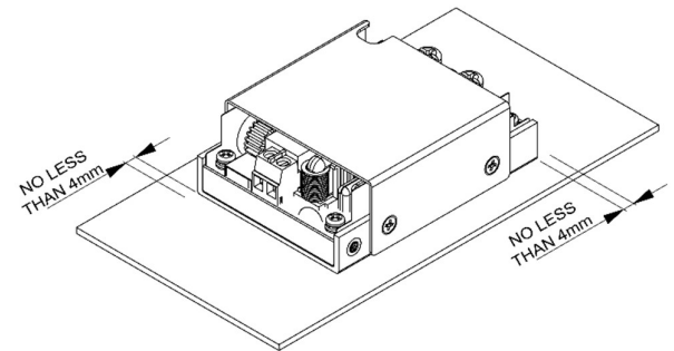
LFM200MXXC Installation Diagram
