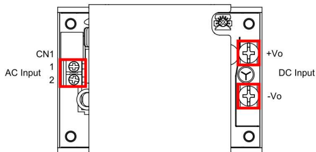
LFM200MXXXC Installation Diagram
