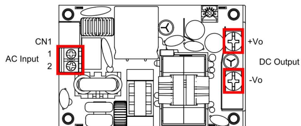
LFM200MXXXB Installation Diagram
