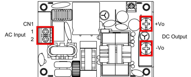
LFM200SXXXB Installation Diagram
