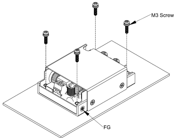
LFM200SXXXC Installation Diagram
