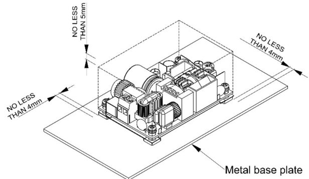
LFM200SXXXB Installation Diagram
