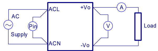
Figure 1. LFM200S Series Test Setup
