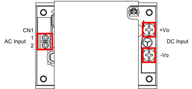
LFM200SXXXC Installation Diagram
