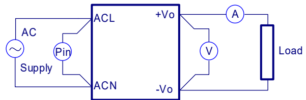
Figure 1. LFM300M Series Test Setup
