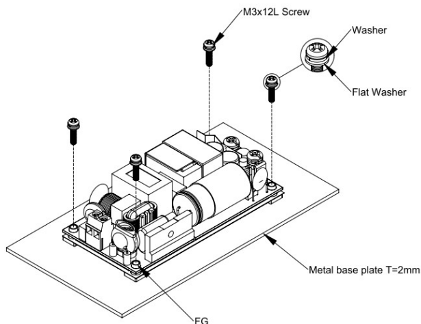
LFM300MXXXB Installation Diagram
