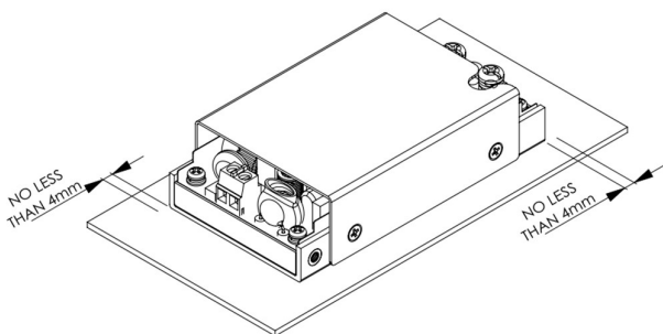
LFM300MXXXC Installation Diagram
