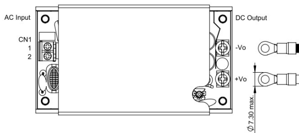
LFM300MXXXC Installation Diagram
