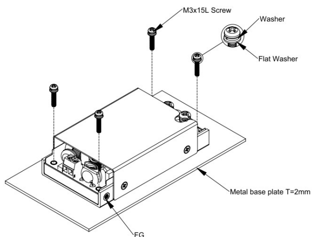
LFM300MXXXC Installation Diagram
