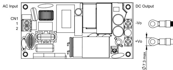
LFM300MXXXB Installation Diagram
