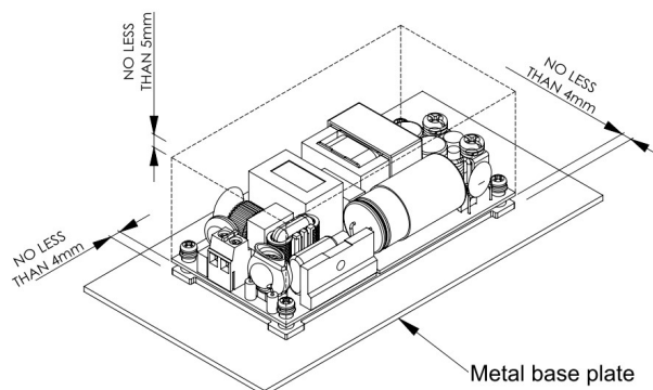
LFM300MXXXB Installation Diagram
