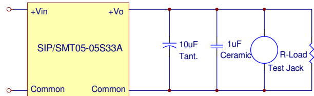
Figure 18. Output Voltage Ripple and Noise Measurement Set-Up
