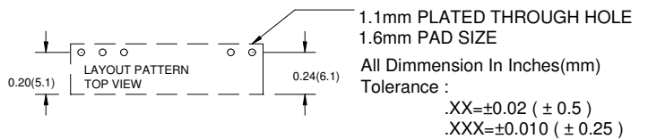
Figure 5. Recommended SIP Footprint
