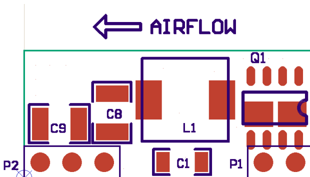
Figure 8. Temperature Measurement Location for SIP
