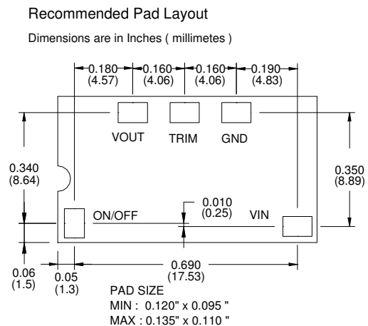
Figure 6. Recommended SMT Footprint (Top View)
