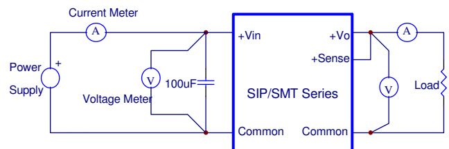
Figure 15. SIP/SMT05 Series Test Setup
