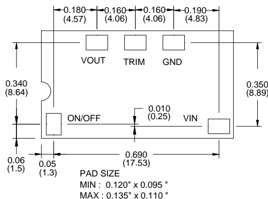
Figure 6. Recommended SMT Footprint (Top View)
