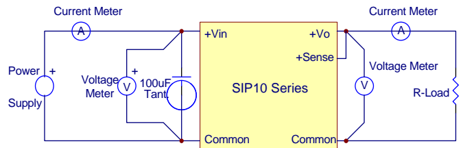
Figure 15. SIP10 Series Test Setup
