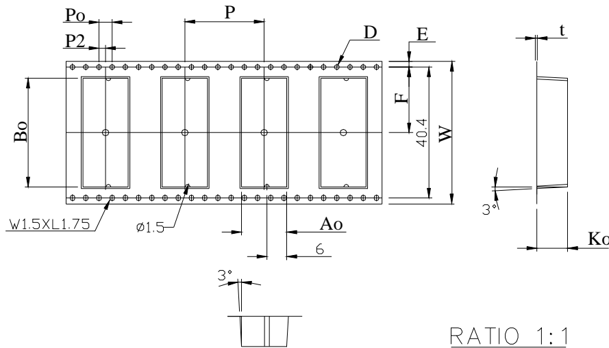
Figure 24 – SMT Tape and Reel Dimensions
