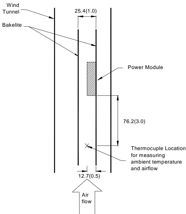
Figure 7. Thermal Test Setup
