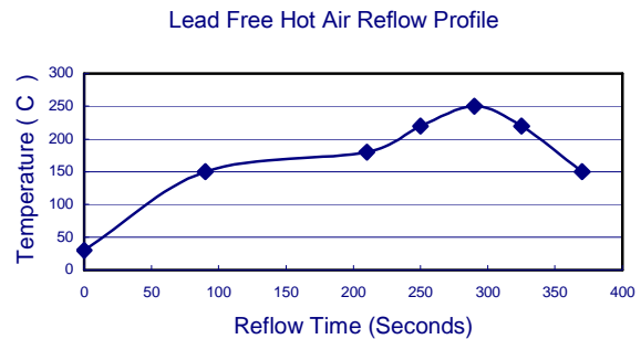
Figure 21 SMT Reflow Profile
