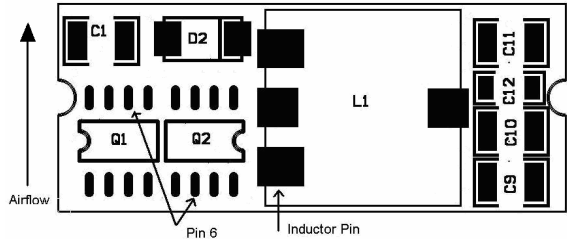
Figure 9. Temperature Measurement Location for SMT
