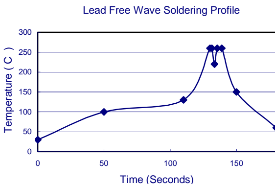
Figure 20 SIP Soldering Profile
