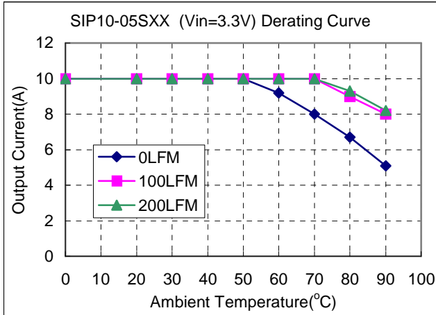
Figure 10. Typical Power De-rating for 3.3V IN
