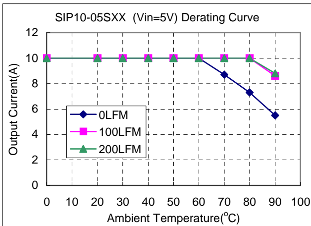
Figure 12. Typical Power De-rating for 5.0V IN
