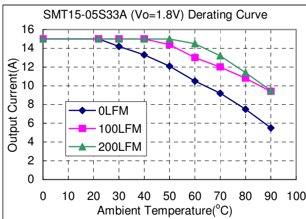
Figure12c. Typical Power De-rating for 5V IN 1.8Vout
