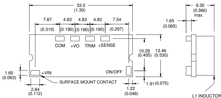
Figure 22 SMT15 Mechanical Outline Diagram
