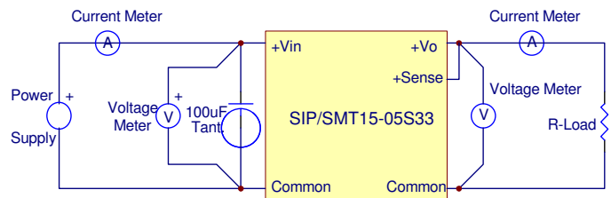
Figure 15. SIP/SMT15 Series Test Setup
