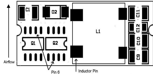
Figure 9. Temperature Measurement Location for SMT
