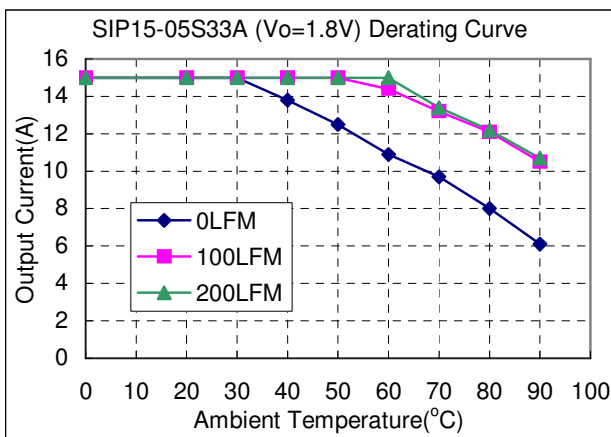
Figure11c. Typical Power De-rating for 3.3V IN 1.8Vout
