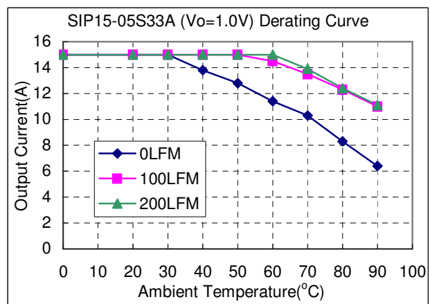
Figure 11f. Typical Power De-rating for 3.3V IN 1.0Vout
