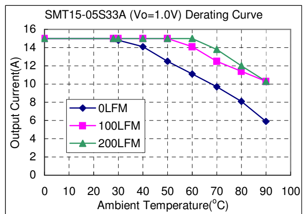
Figure 12f. Typical Power De-rating for 5V IN 1.0Vout
