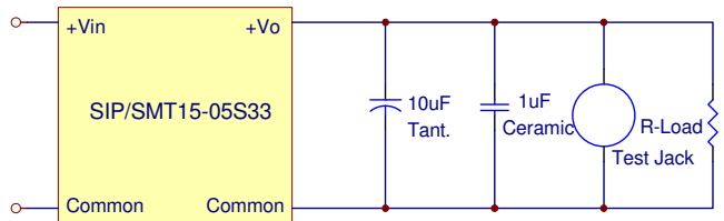
Figure 19. Output Voltage Ripple and Noise Measurement Set-Up
