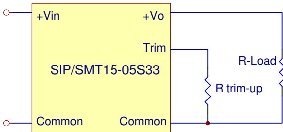
Figure 17. Trim-up Voltage Setup
