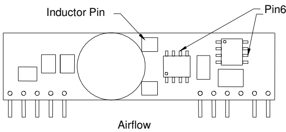
Figure 8. Temperature Measurement Location for SIP
