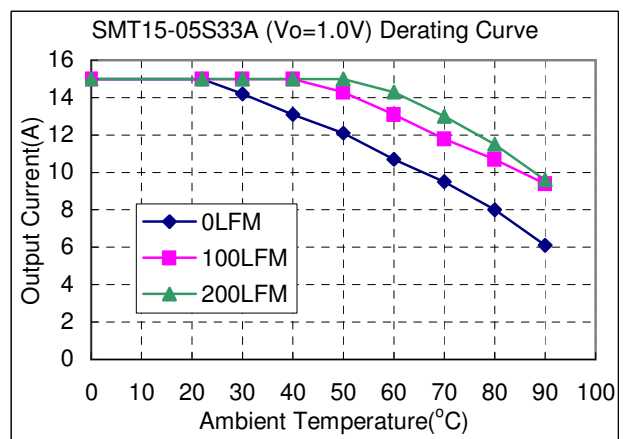
Figure 13f. Typical Power De-rating for 3.3V IN 1.0Vout
