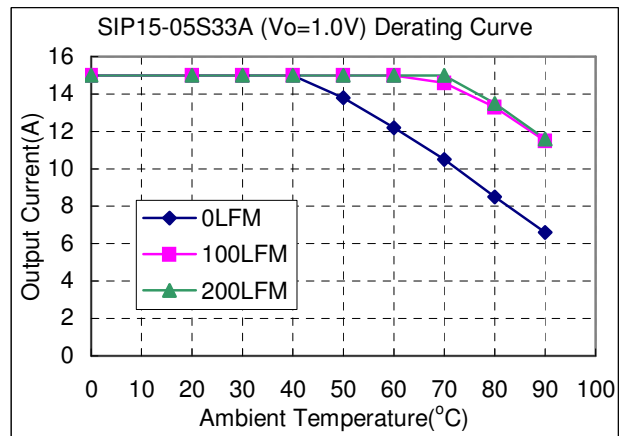
Figure 10f. Typical Power De-rating for 5.0V IN 1.0Vout
