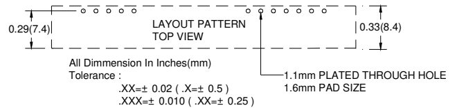
Figure 8. Recommended SIP Footprint
