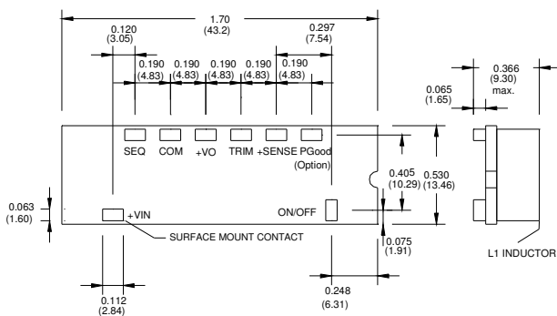
Figure 22 SMT20W-12 Mechanical Outline Diagram
