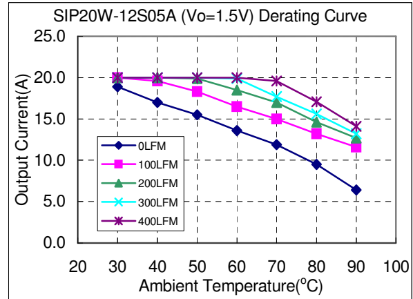
Figure 13f. Typical Power De-rating for 12V IN 1.5Vout
