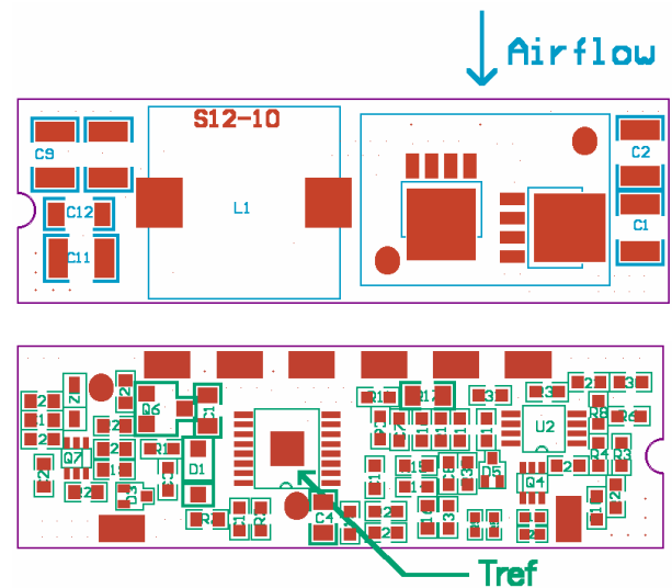
Figure 12. Temperature Measurement Location for SMT
