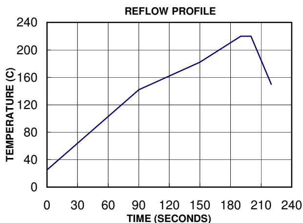
Figure 20 SMT Reflow Profile
