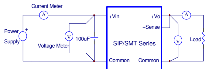
Figure 16. SIP/SMT20W Series Test Setup
