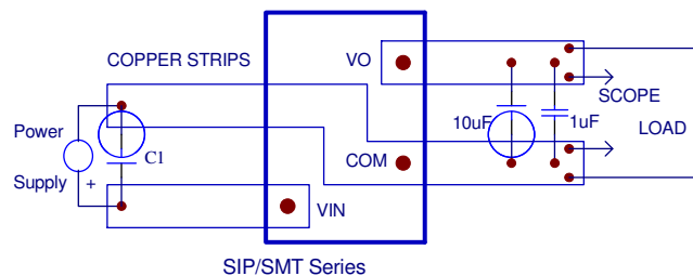
Figure 19. Output Voltage Ripple and Noise Measurement Set-Up
