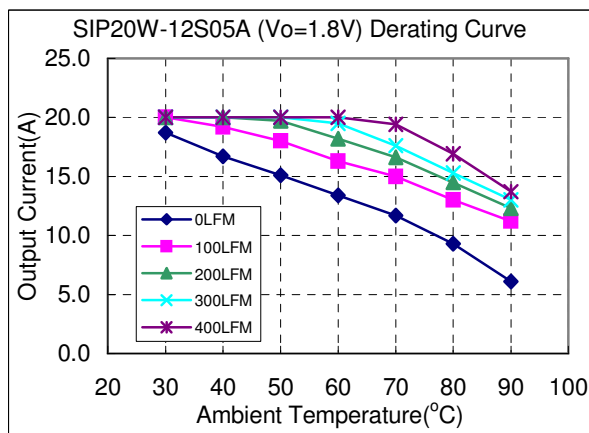
Figure13e. Typical Power De-rating for 12V IN 1.8Vout
